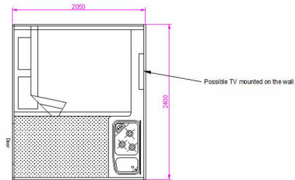
FLOOR PLAN
